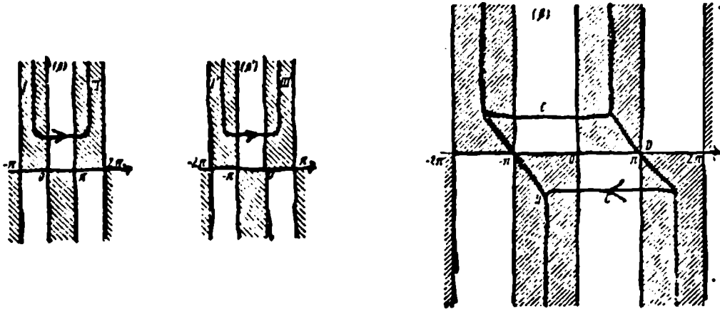
Figure 2. The integration contours Figure 3. The integration contour in Equation (1.28).
