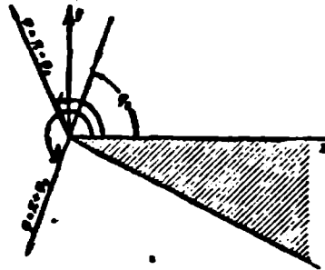
Figure 5. Diffraction of a plane wave by a wedge. The plane wave irradiates only one face of the wedge. \phi_0 is the angle of incidence. The line \phi = \pi - \phi_0 is the boundary of the reflected plane wave, and the line \phi = \pi + \phi_0 is the boundary of the shadow.
